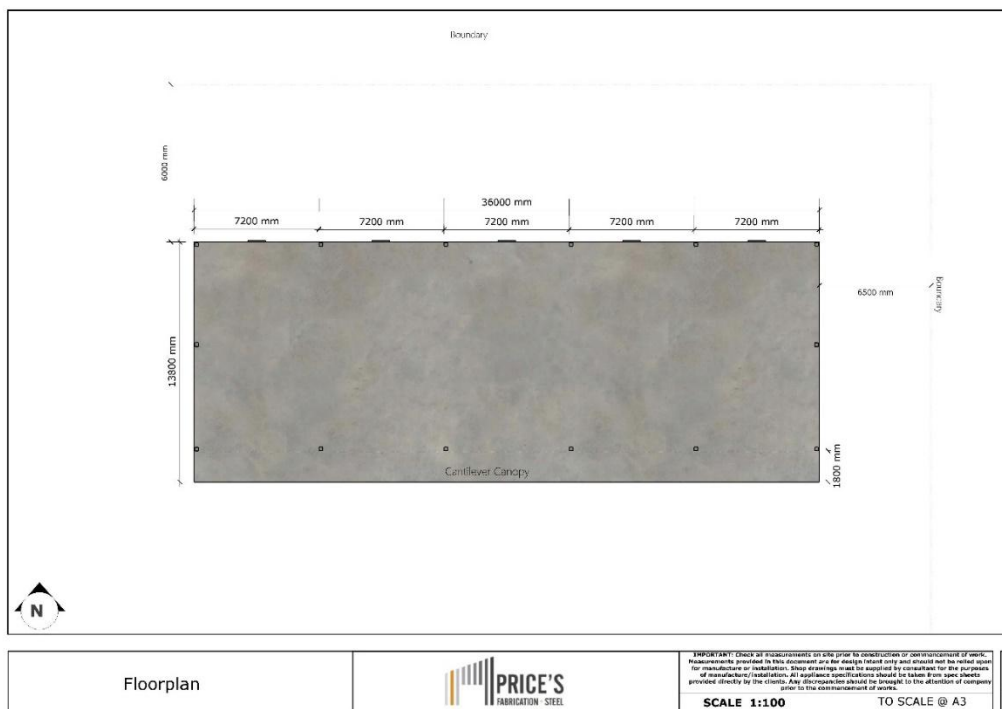
Figure 4 & 5- 3D and elevation plans
